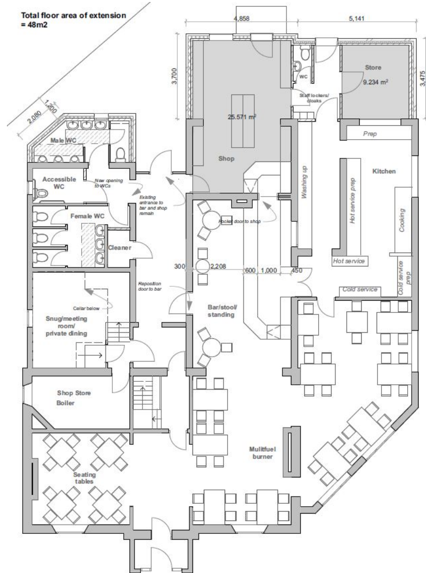
Proposed Layout
