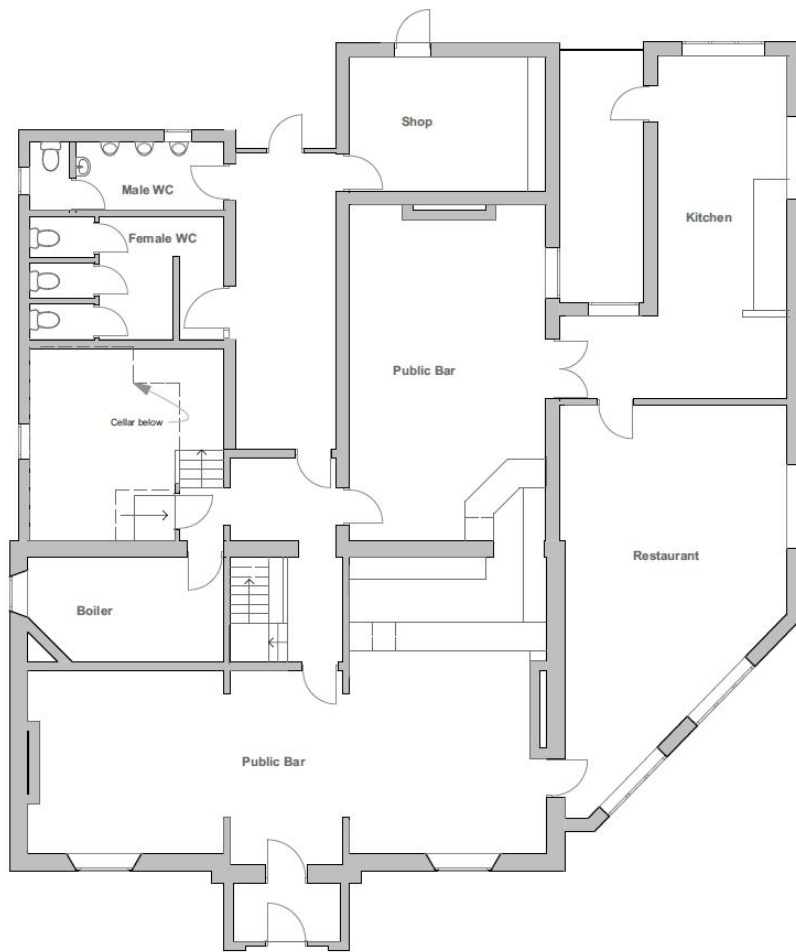
Original Layout
